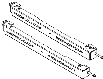
Left and Right Mounting Bracket -BB (Qty 1 Each)
